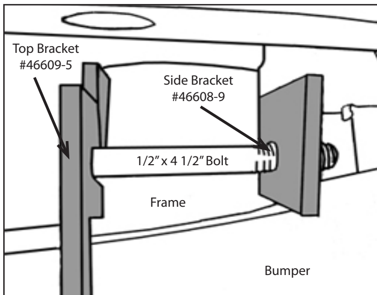
Driver Side top of frame, with Brackets #46609-5 and #46608-9
